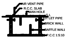
SECTION ON SEP.TANK
