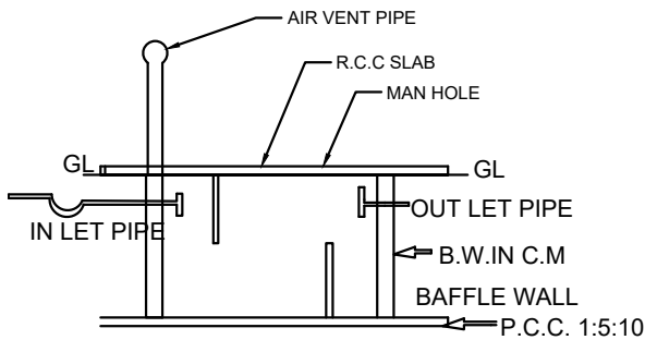
SECTION ON SEPTIC TANK
