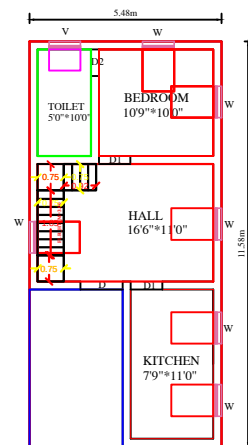
PROPOSED G.FLOOR PLAN
