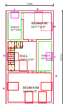
PROPOSED F. FLOOR PLAN
