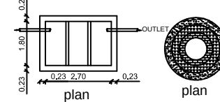
SEPTIC TANK LEACH WELL DETAIL
