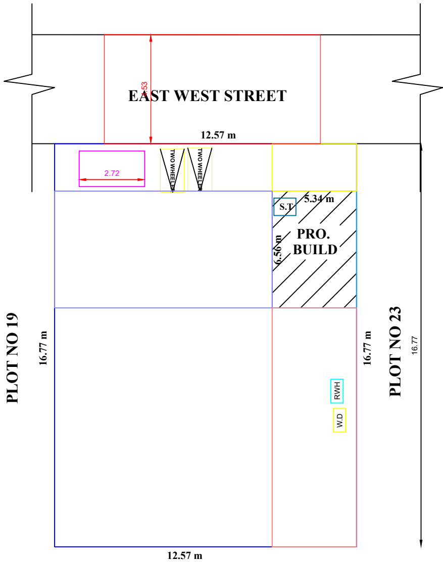
SITE PLAN
