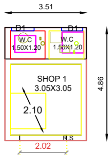
FLOOR PLAN
