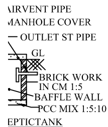
SECTION OF BS
