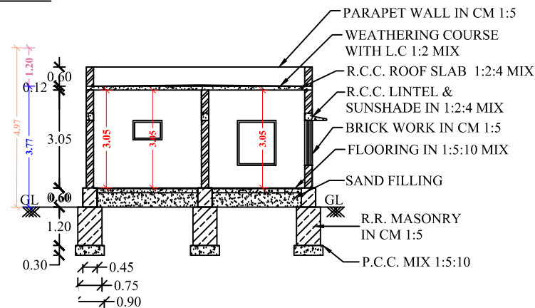
SECTION OF "AB"
