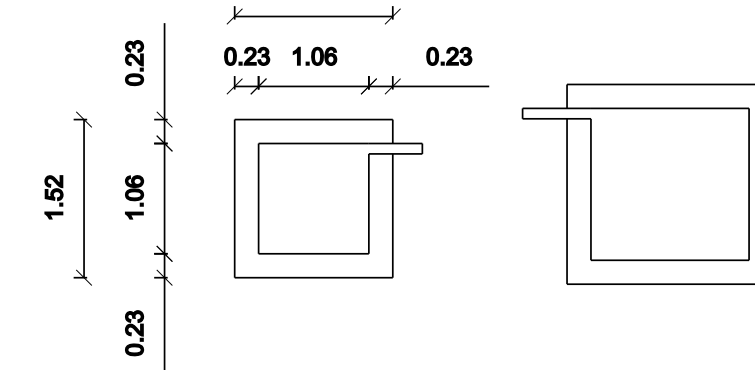
DETAILS OF FILTER BED & WELL
