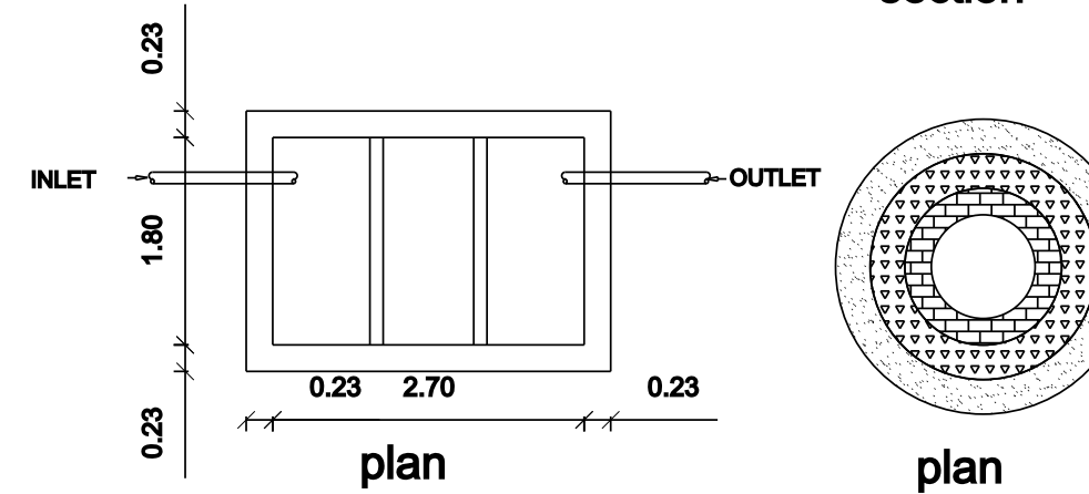
SEPTIC TANK
