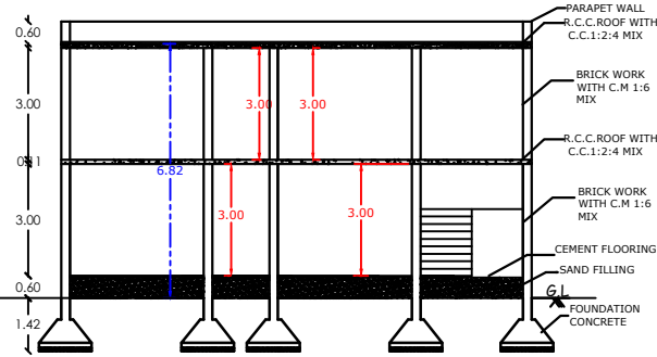
SECTION ON "BA"
