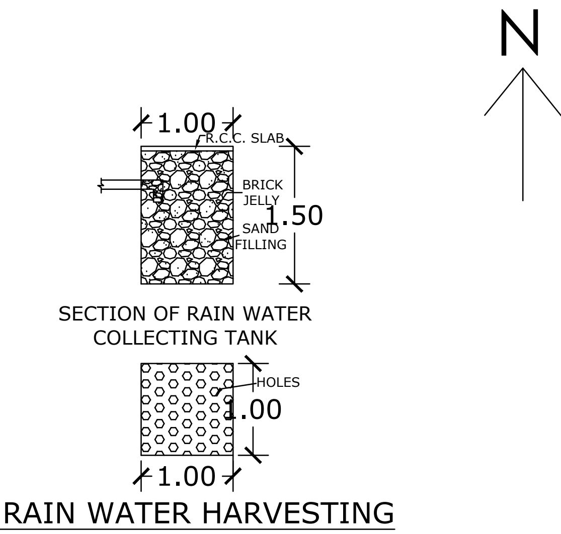
RAIN WATER HARVESTING
