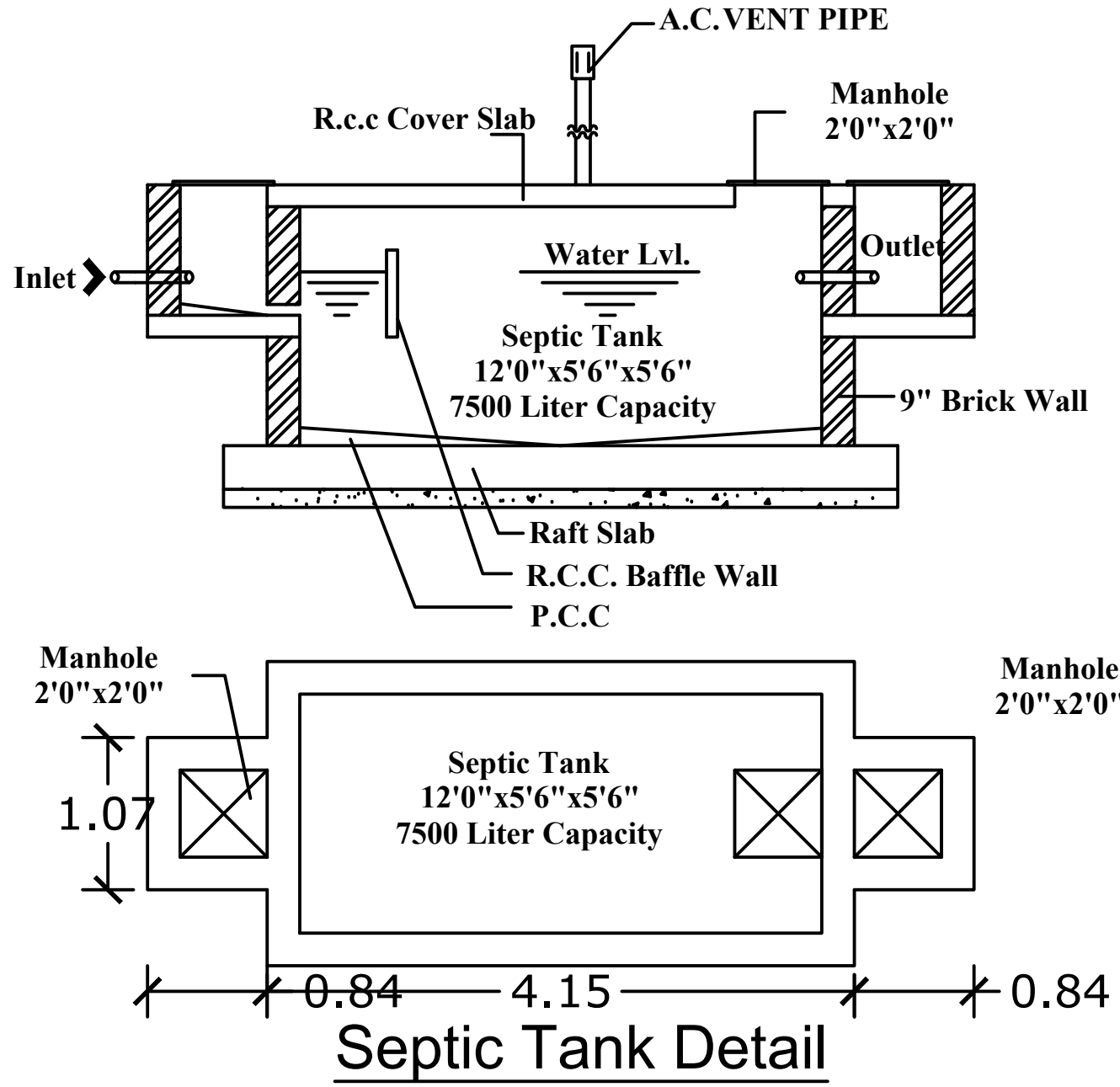
Septic Tank Detail
