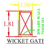
WICKET GATE
