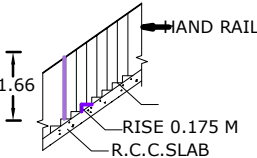
STAIRCASE
