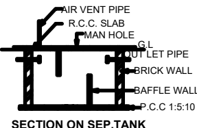
SECTION ON SEP.TANK
