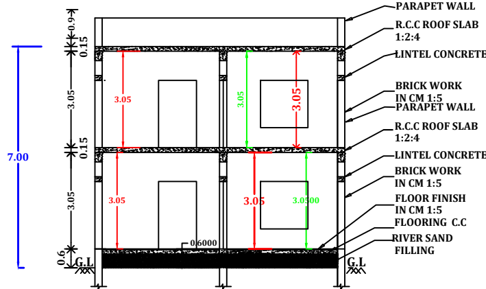
SECTION ON AA1
