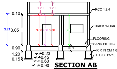
SECTION AB
