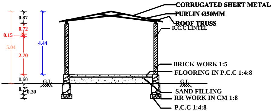
"SECTION "AB"
