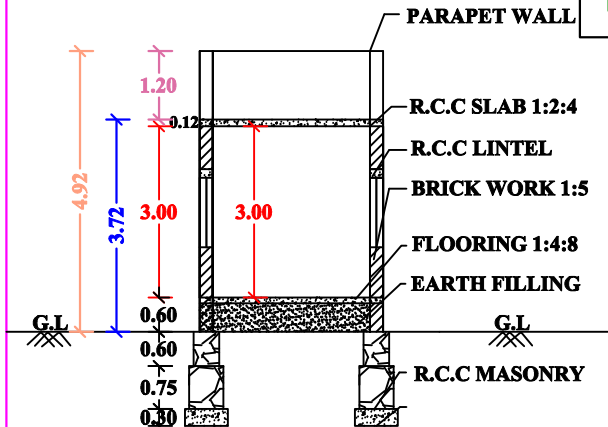
"SECTION "AB"
