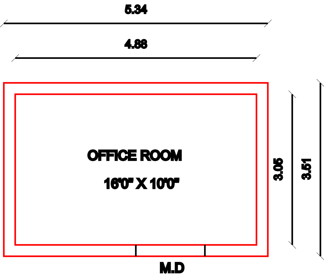
PLAN
