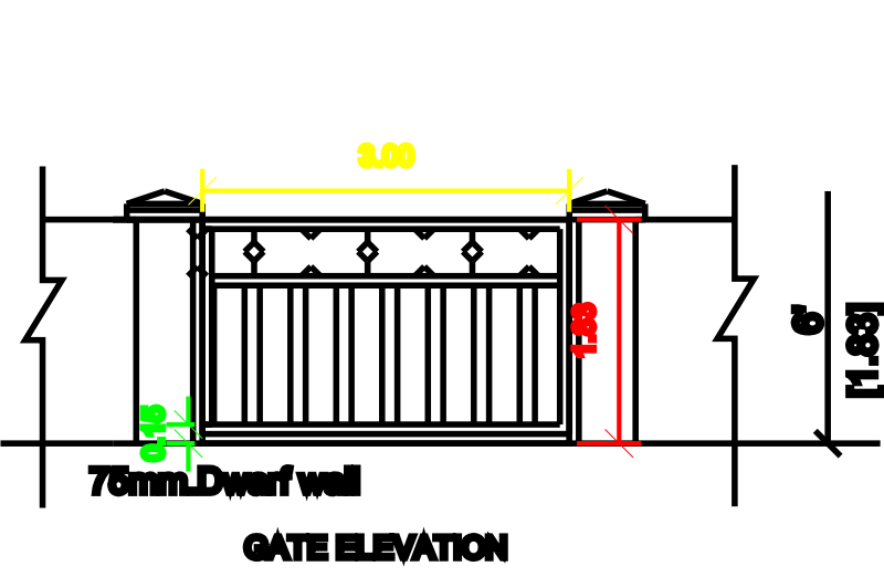
GATE ELEVATION
