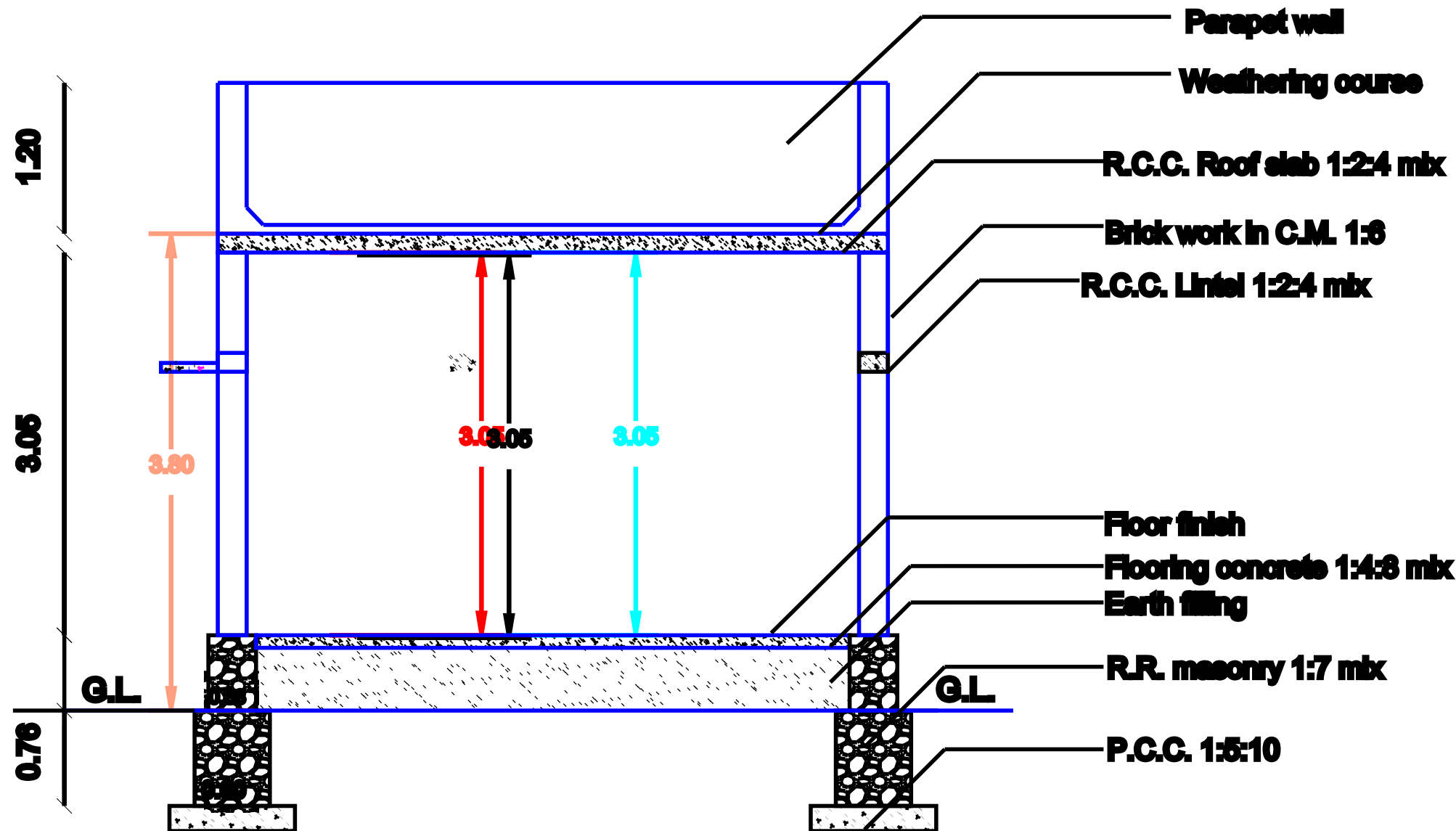
SECTION AB
