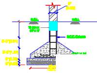
FOUNDATION
