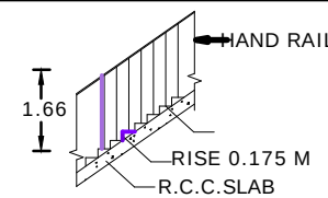
STAIRCASE
