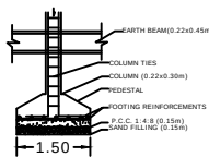
FOUNDATION DETAILS
