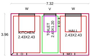
PROPOSED GF PLAN
