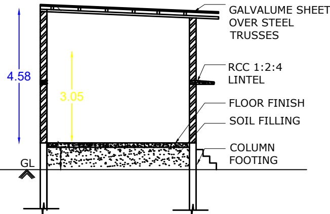
SECTION
