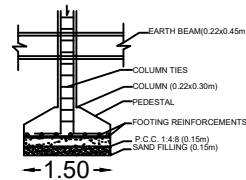
FOUNDATION DETAILS
