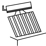
SOLAR SYSTEM
