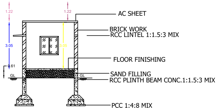
SECTION AB
