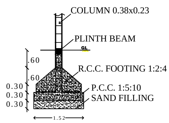
COLUMN DETAILS
