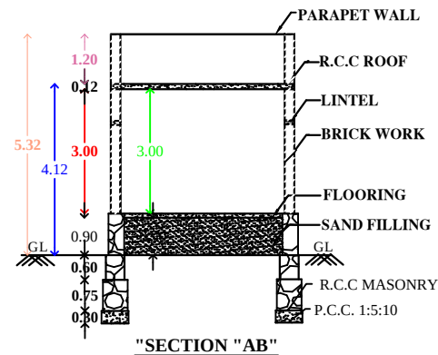
"SECTION "AB"
