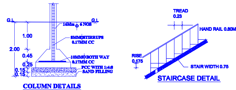
COLUMN DETAILS
