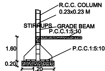
COLUMN DETAIL
