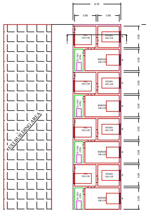
EXI.GROUND FLOOR PLAN
