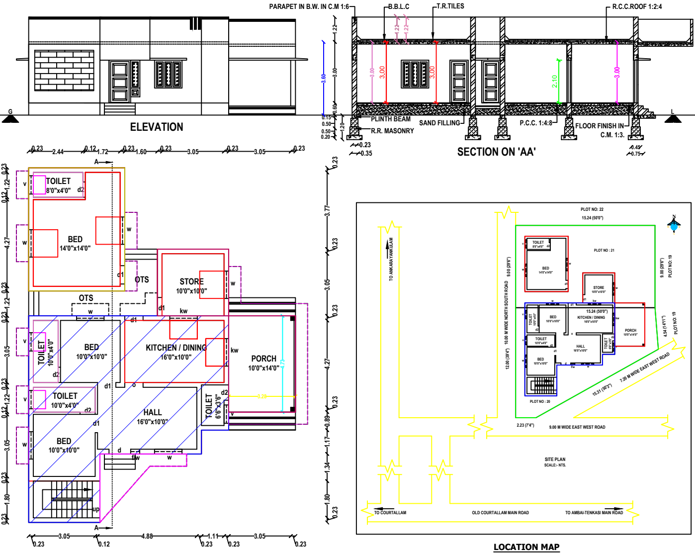
PLAN - GROUND FLOOR RESIDENCE EXISTING & ADDITION
