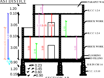
SECTION AB
