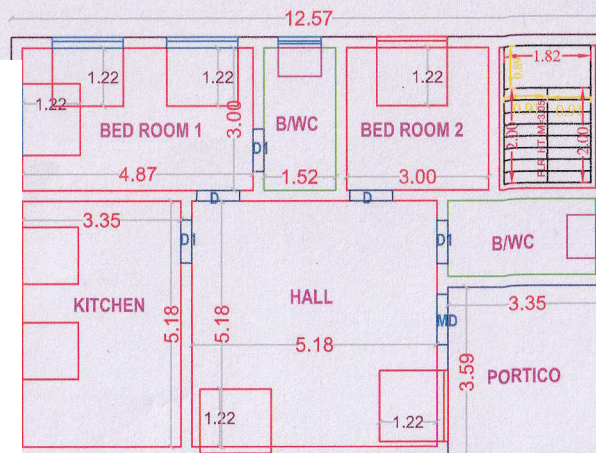
PLAN - GROUND FLOOR ( PRO.BUILDING )
