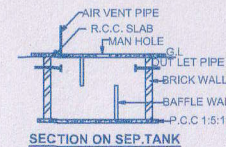
SECTION ON SEP.TANK
