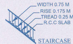
STAIRCASE
