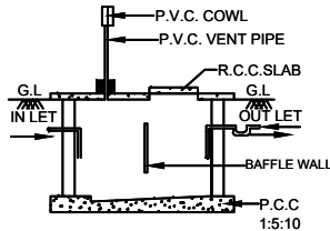
SEC. OF SEPTIC TANK
