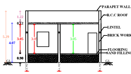
"SECTION "AB"
