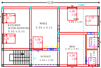
PRO.GROUND FLOOR PLAN
