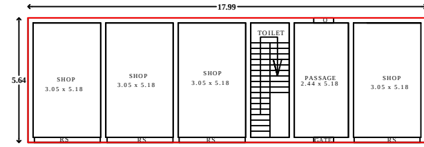
EXG.GROUND FLOOR PLAN
