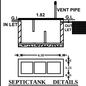
SEPTICTANK DETAILS
