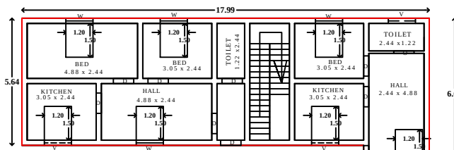
EXG.FIRST FLOOR PLAN
