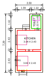
PRO.GROUND FLOOR PLAN
