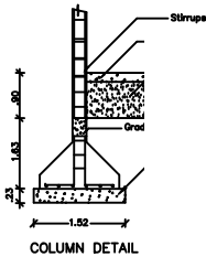
COLUMN DETAIL
