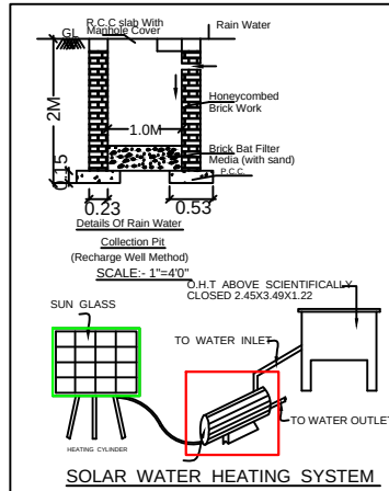
SOLAR WATER HEATING SYSTEM
