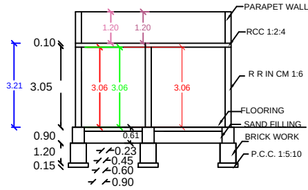
SECTION AB
