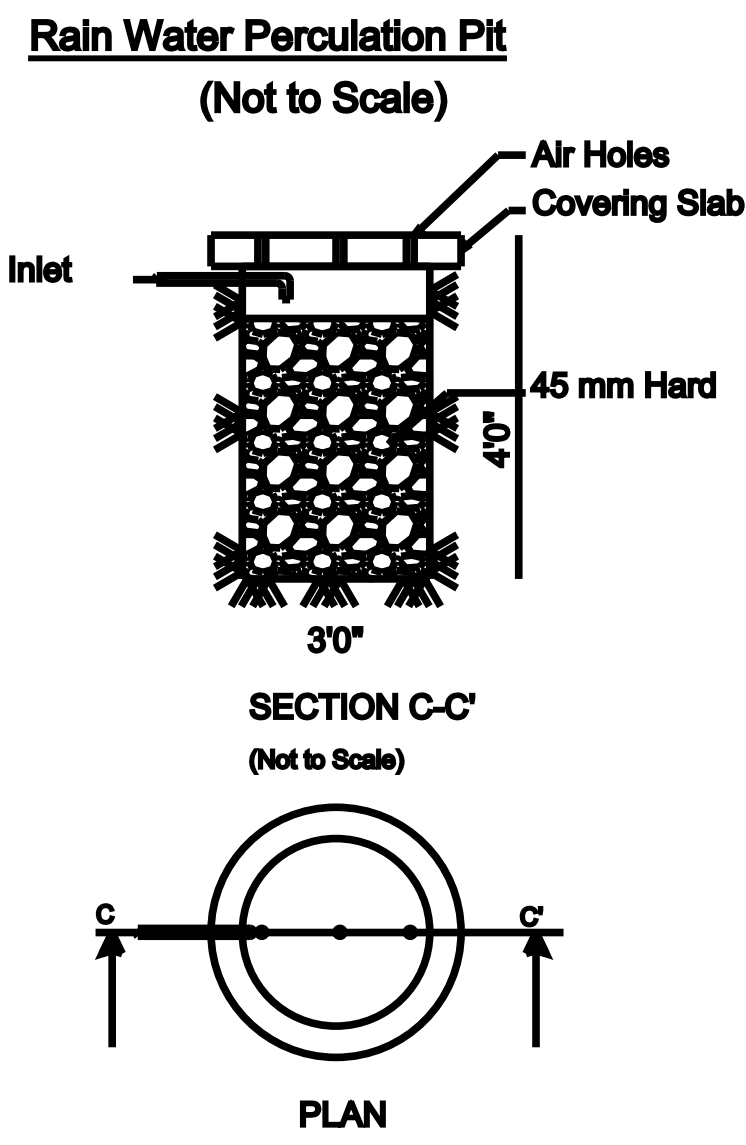
PLAN
