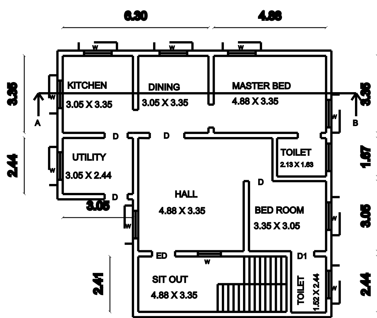
PLAN
