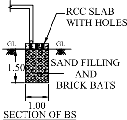
SECTION OF BS PLAN OF RAINWATER HARVEST TANK
