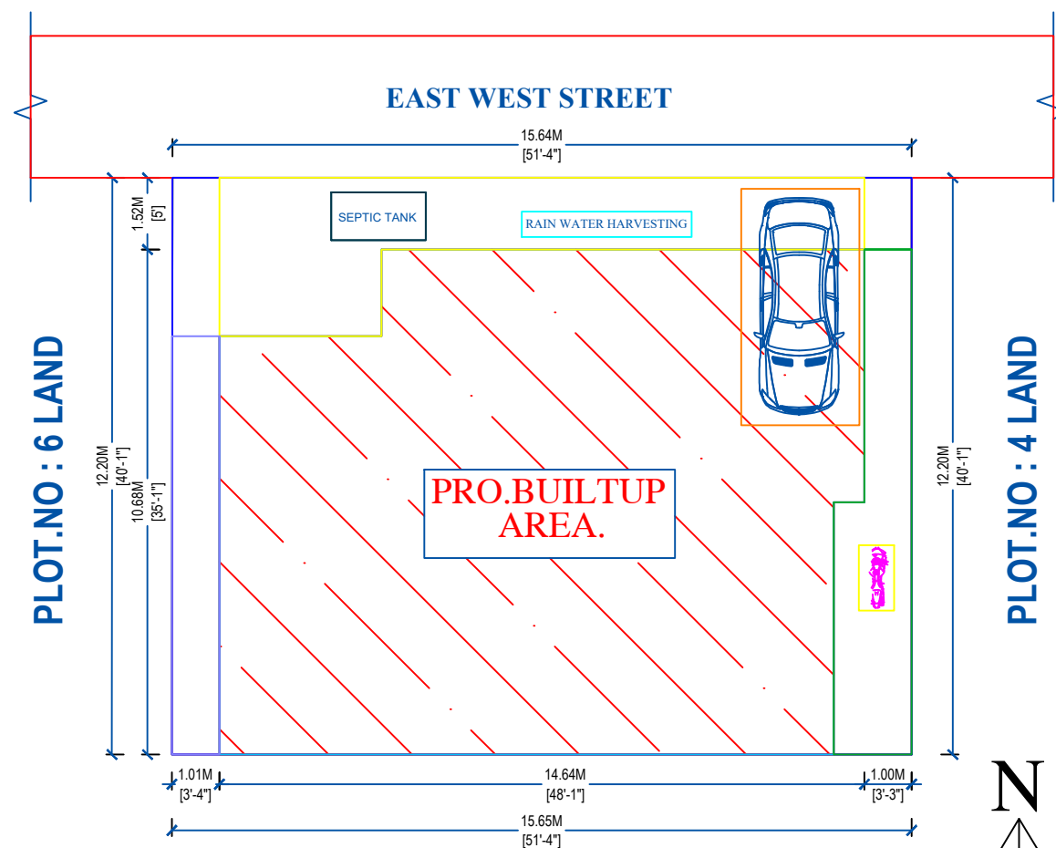
PLOT.NO : 17 LAND SITE PLAN SCALE:- 1:100
