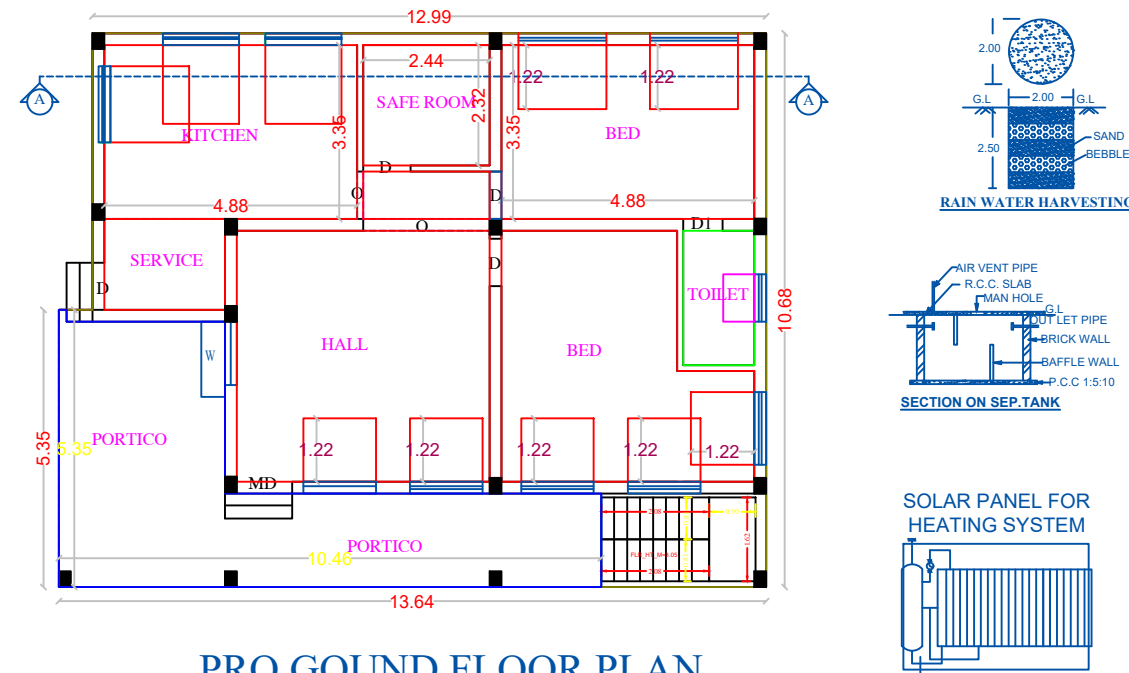
PRO.GOUND FLOOR PLAN ( PROPOSED )
