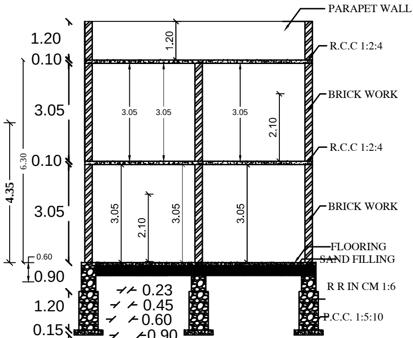
SECTION AB
