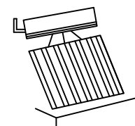
SOLAR SYSTEM
