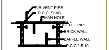
SECTION ON SEP.TANK
