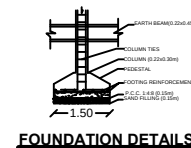
FOUNDATION DETAILS
