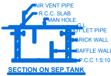
SECTION ON SEP. TANK
