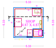
FLOOR PLAN
