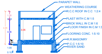
SECTION ON 'AZ'
