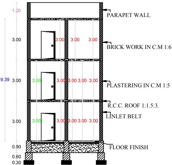
SECTION AB
