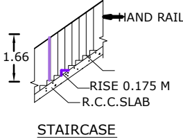
STAIRCASE
