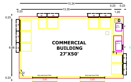
PRO GROUND FLOOR COMMERCIAL PLAN
