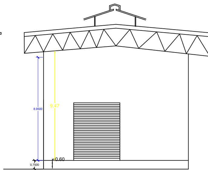
SECTION ON " XY "
