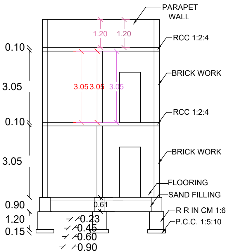
SECTION AB
