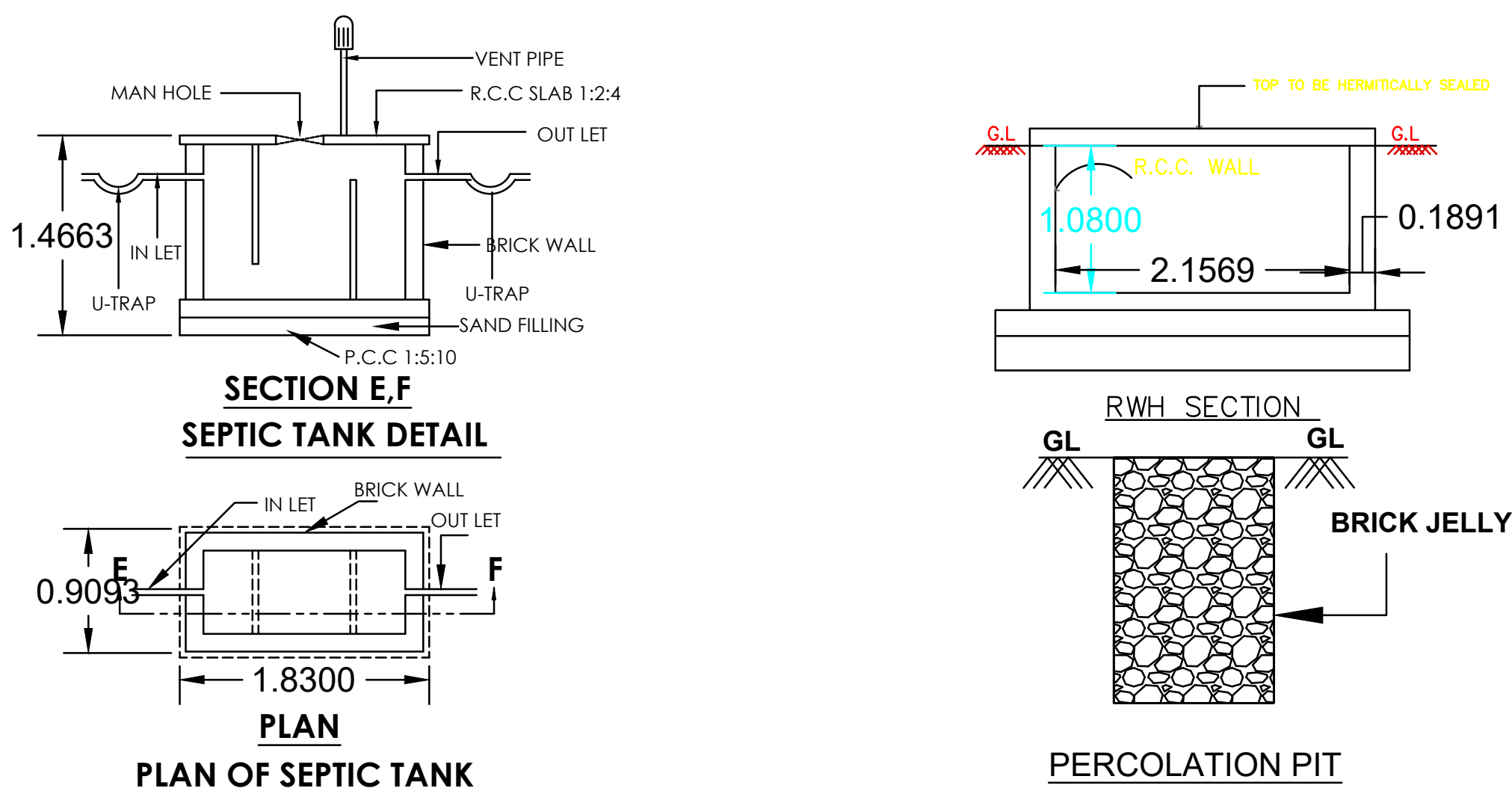
PERCOLATION PIT
