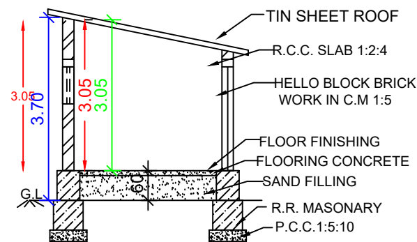
SECTION ON - BB
