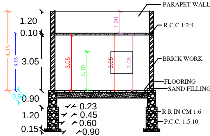
SECTION AB
