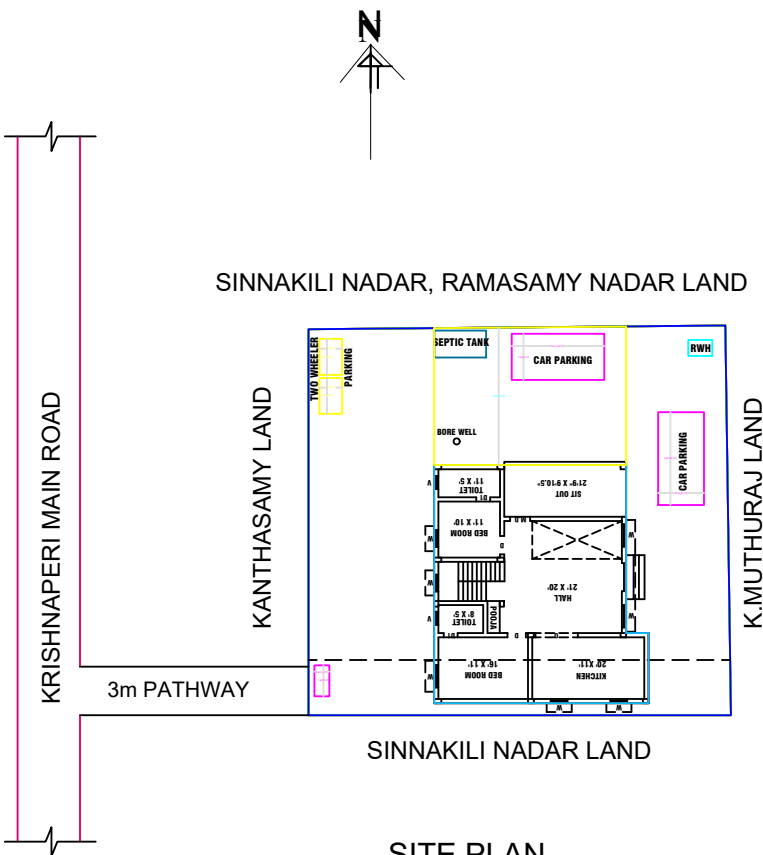
SITE PLAN SCALE 1:50
