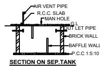
SECTION ON SEP.TANK
